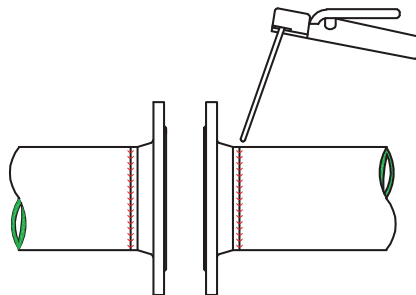
5- Fully weld flanges to the pipes.
